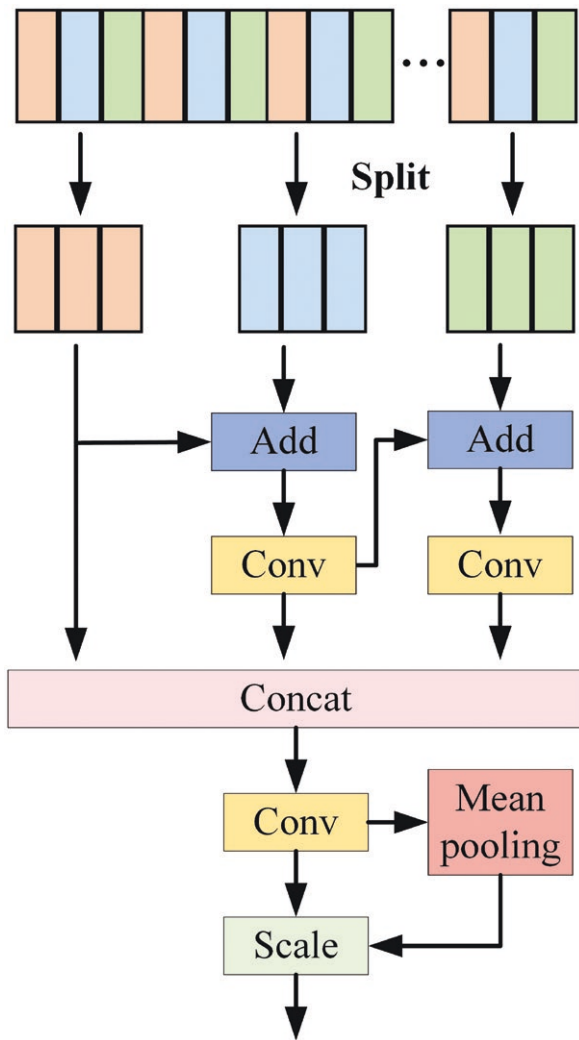
Figure 5. MSFCA model structure.
