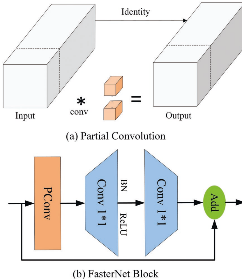
Figure 3. FasterNet Block model structure.
