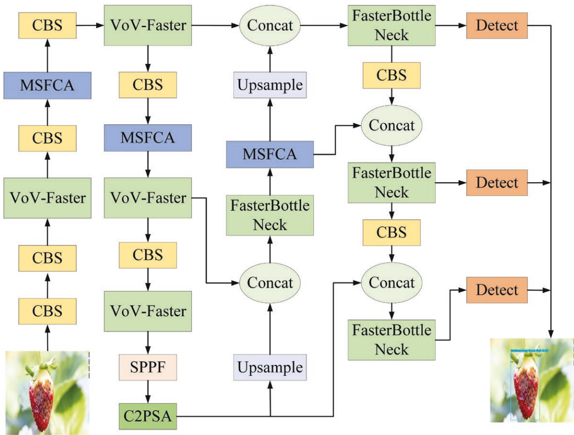
Figure 6. YOLO11-Strawberry model structure diagram.
