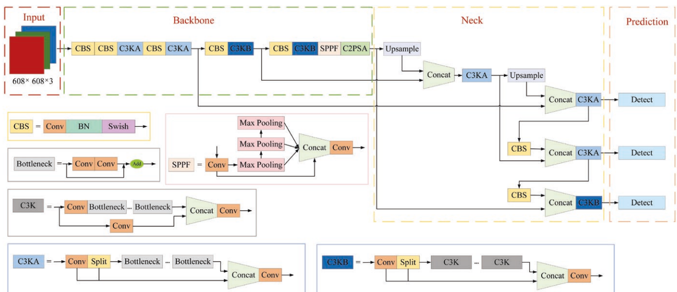
Figure 2. YOLO11 model structure.
