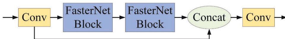
Figure 4. VoV-Faster model structure.
